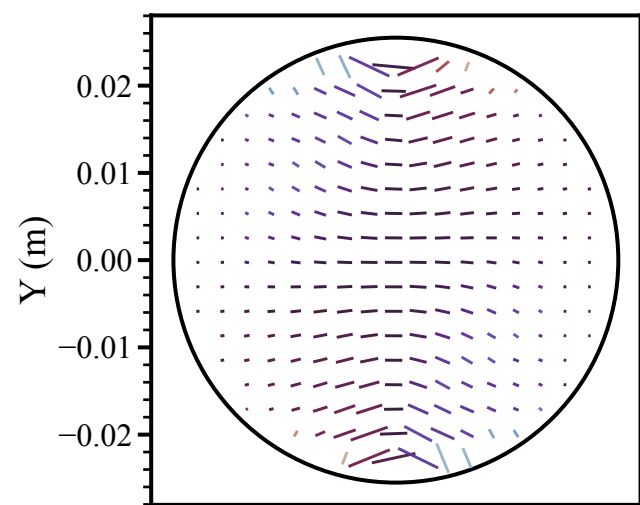
Augen gneiss ( 90^\circ )
