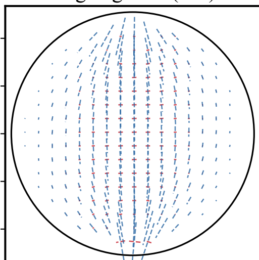
Augen gneiss (45°)
