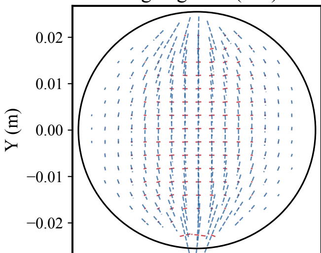
Augen gneiss (30°)
