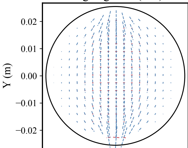
Augen gneiss (60°)
