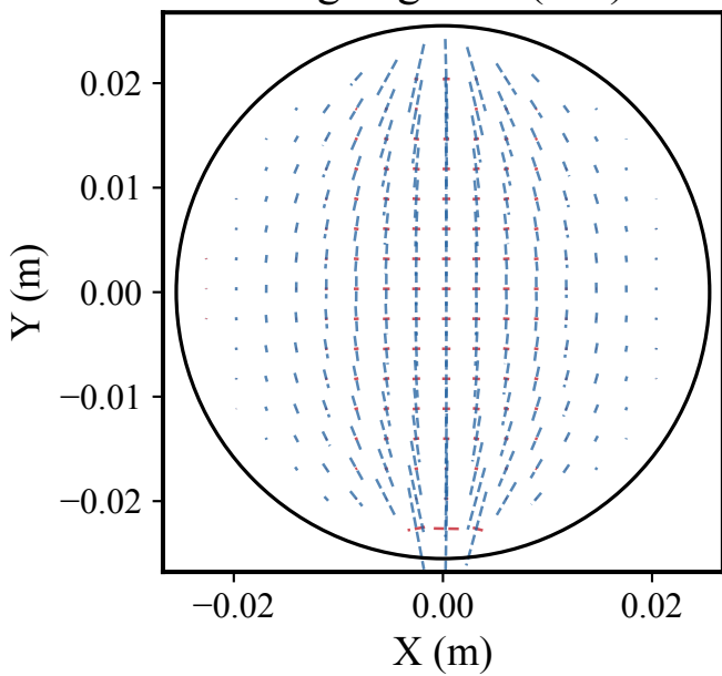
Augen gneiss (90°)
