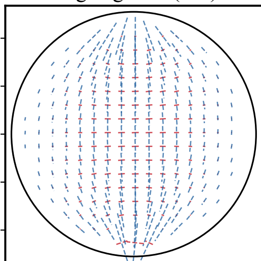
Augen gneiss (15°)
