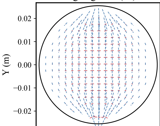
Augen gneiss (0°)
