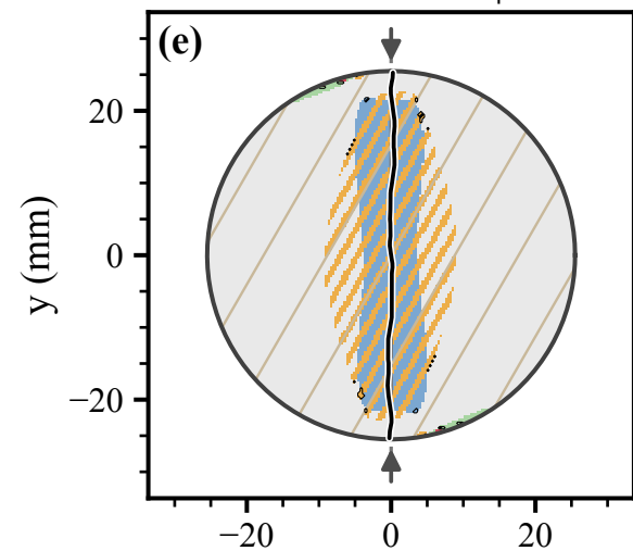
Psammitic schist, \alpha_{\text{exp}} = 60^\circ
