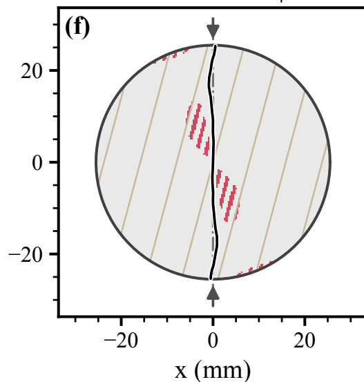
Psammitic schist, \alpha_{\text{exp}} = 75^\circ
