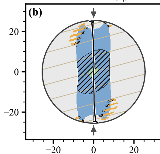
Psammitic schist, \alpha_{\text{exp}} = 15^\circ
