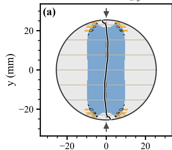
Psammitic schist, \alpha_{\text{exp}} = 0^\circ
