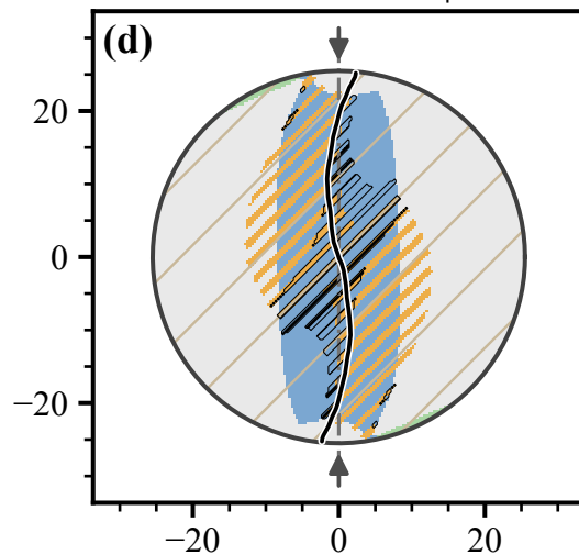
Psammitic schist, \alpha_{\text{exp}} = 45^\circ
