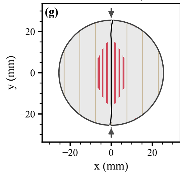
Psammitic schist, \alpha_{\text{exp}} = 90^\circ
