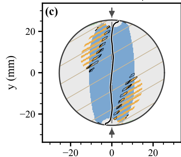
Psammitic schist, \alpha_{\text{exp}} = 30^\circ
