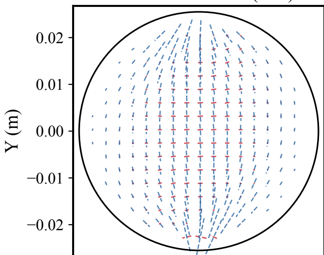
Psammitic schist (30°)
