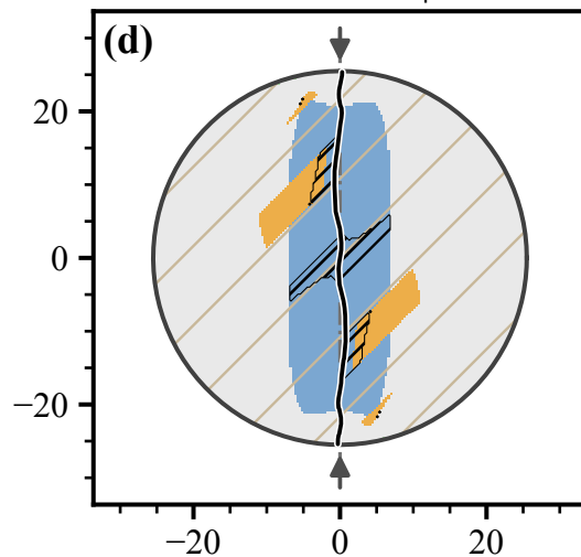
Augen gneiss, \alpha_{\text{exp}} = 45^\circ
