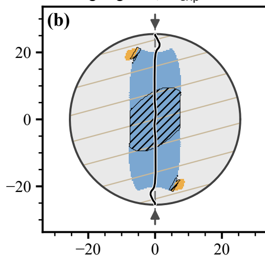
Augen gneiss, \alpha_{\text{exp}} = 15^\circ
