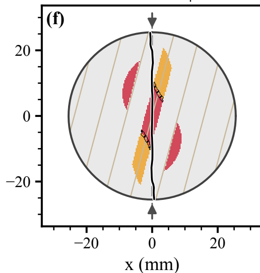
Augen gneiss, \alpha_{\text{exp}} = 75^\circ
