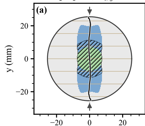
Augen gneiss, \alpha_{\text{exp}} = 0^\circ
