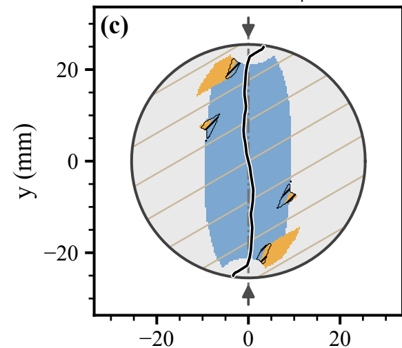
Augen gneiss, \alpha_{\text{exp}} = 30^\circ
