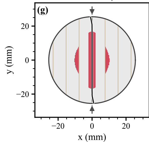
Augen gneiss, \alpha_{\text{exp}} = 90^\circ
