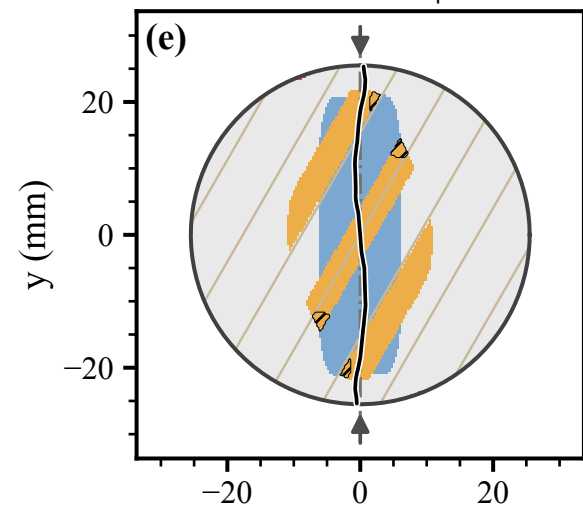
Augen gneiss, \alpha_{\text{exp}} = 60^\circ
