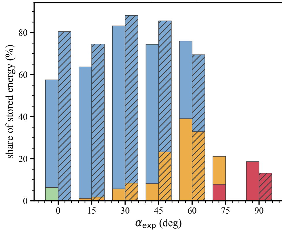
Thrust (-0.50 MPa)
