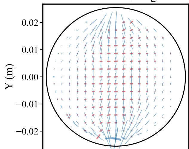
Psammitic schist | Angle=60°
