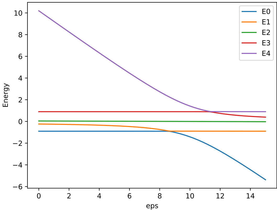
Hamiltonian eigenenergies
