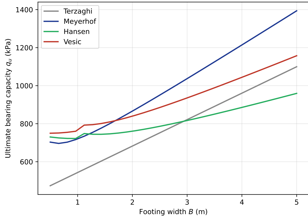
q_u vs B — c = 0 , \phi = 30^\circ , D_f = 1 m, \gamma = 18 kN/m 3
