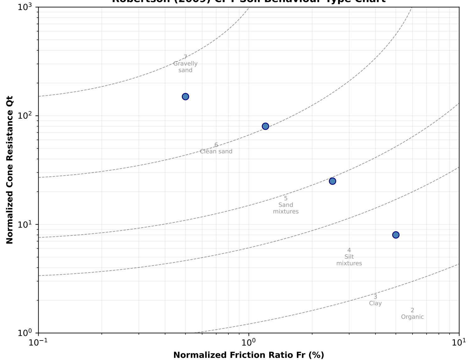
Robertson (2009) CPT Soil Behaviour Type Chart
