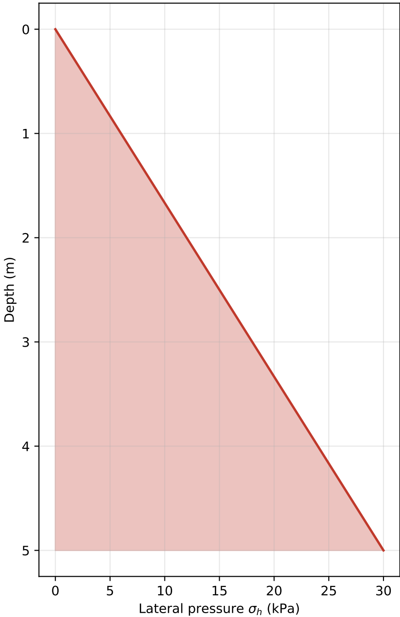
Active earth pressure ( K = 0.333 )
