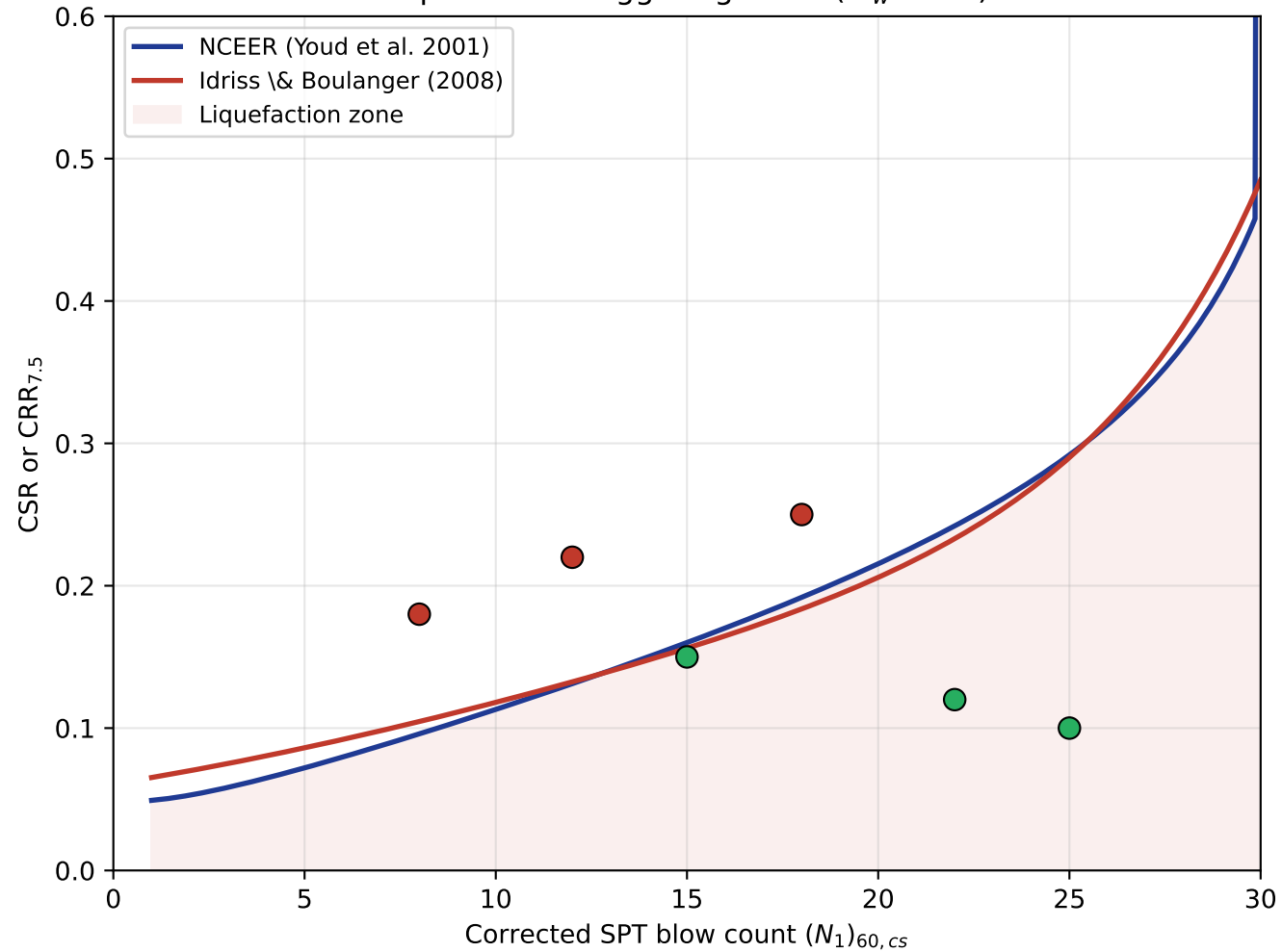
Liquefaction triggering chart ( M_w = 7.5 )
