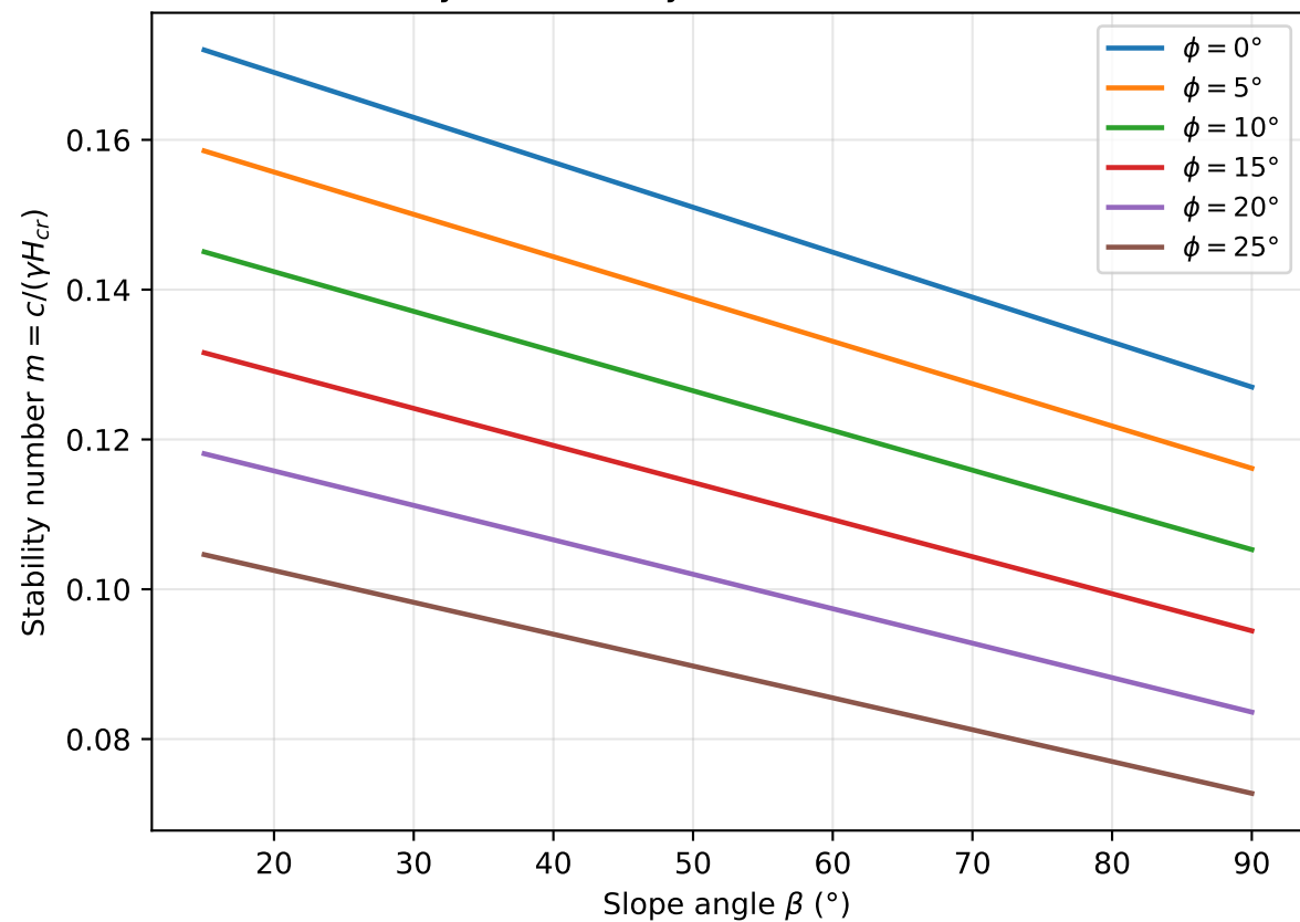
Taylor's stability number (toe circles)
