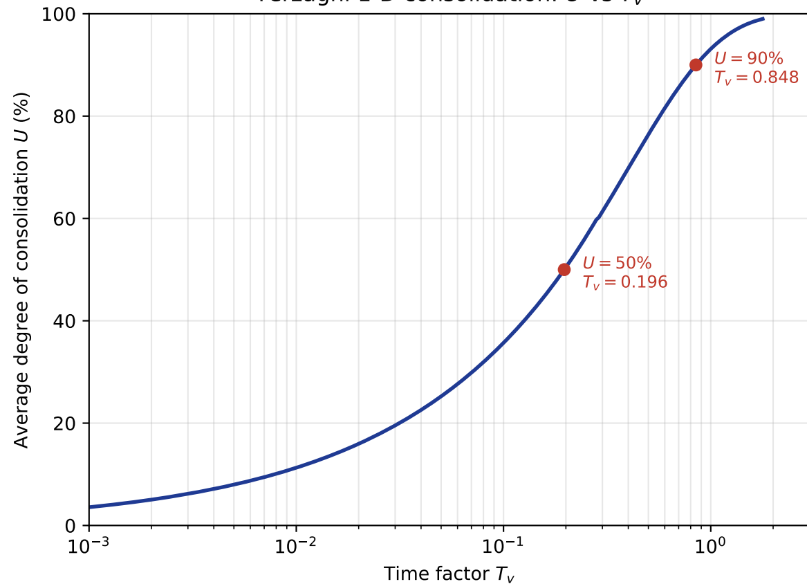
Terzaghi 1-D consolidation: U vs T_v
