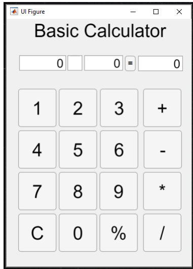
Startup Screen
