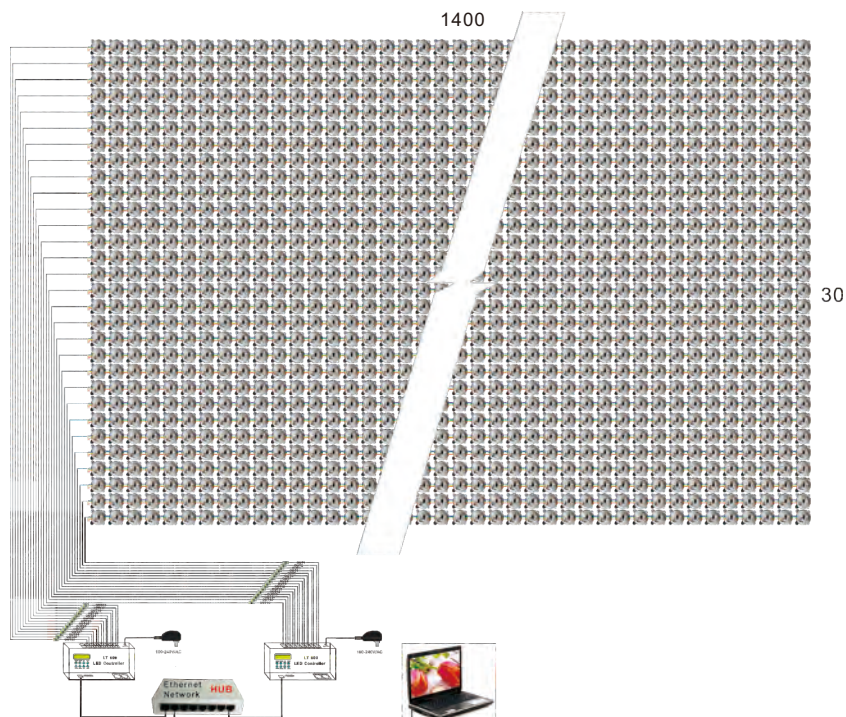
Spot Light Wiring Diagram
