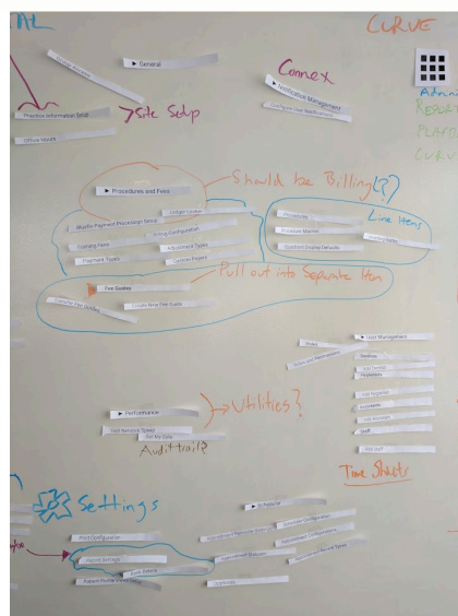
WORKFLOW DEFINITION
