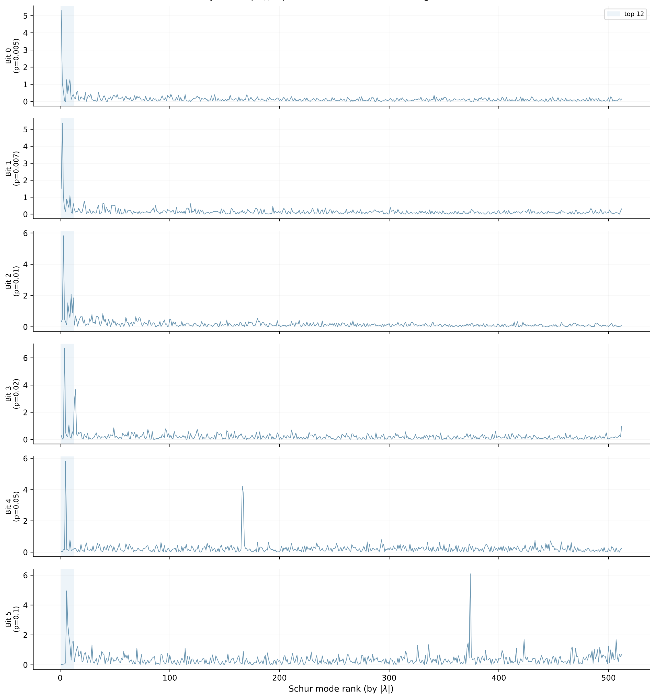
A3 profile: |W_{\text{out}} Q| across all Schur modes — g = 0.5
