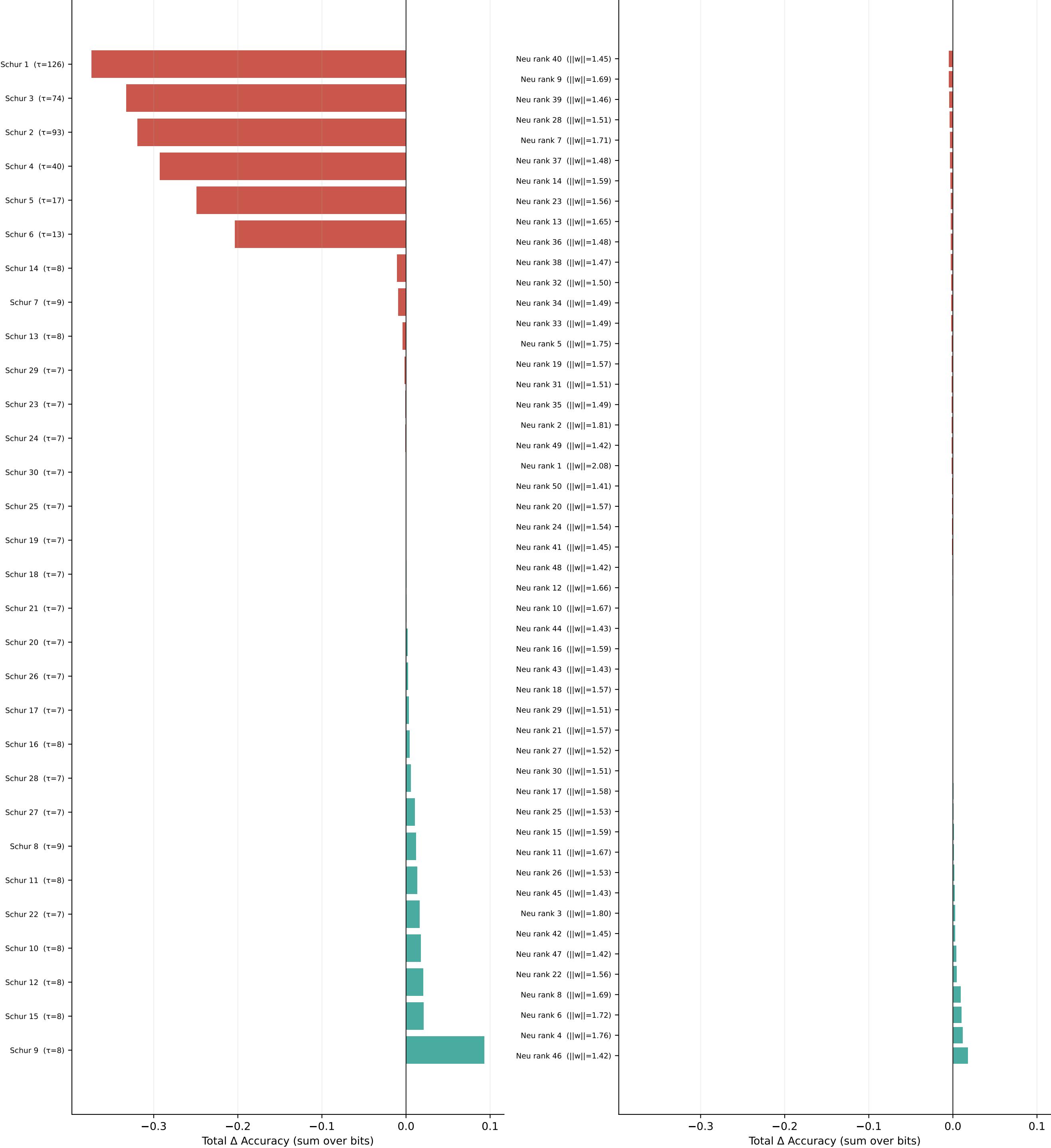
Schur modes (top 30, sorted by drop)
