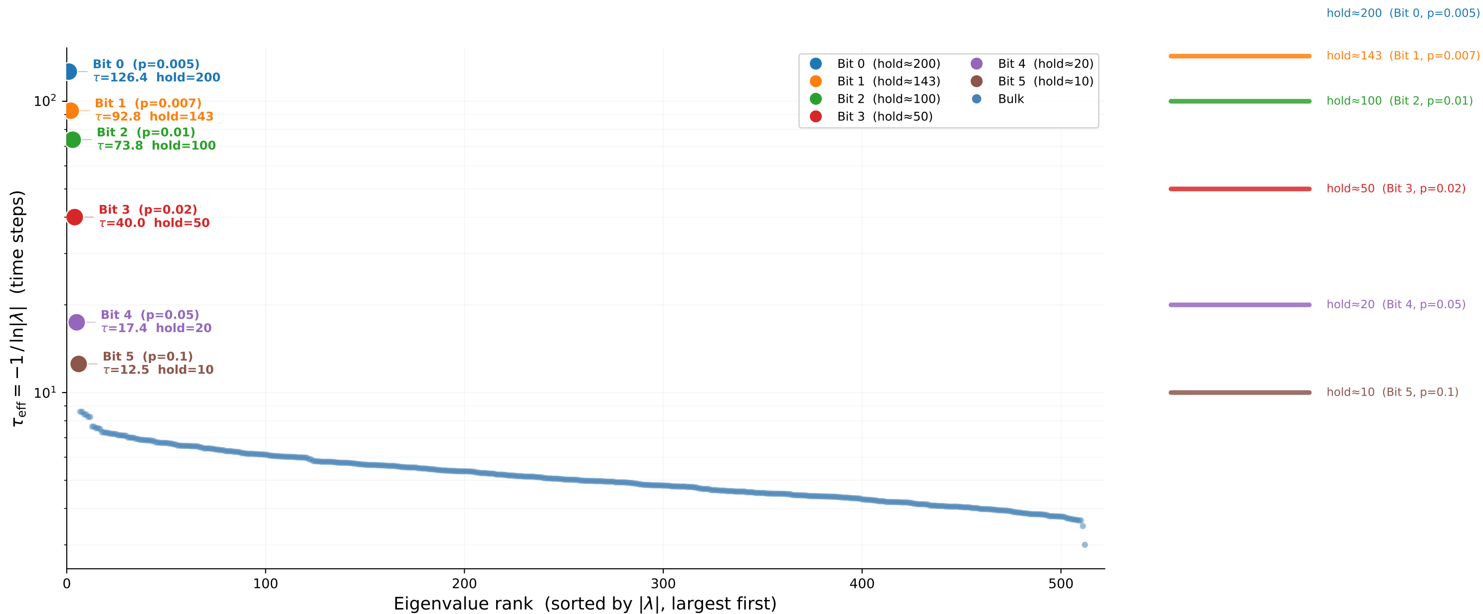
Effective Timescale Scree — g = 0.5 , N = 512 neurons (dominant: correlation)
