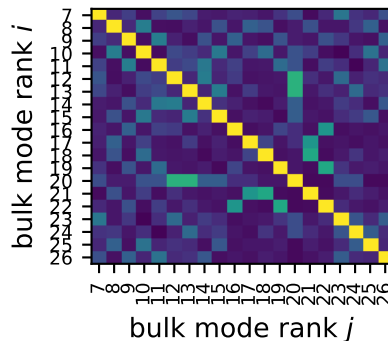
|v_i^H v_j| — top 20 bulk modes (ranks 7...26)
