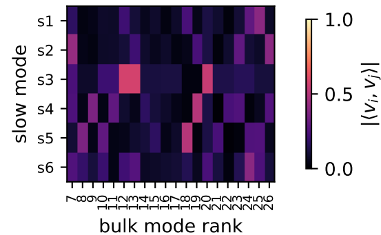
slow \times bulk: |v_s^H v_b| (top 20 bulk modes)
