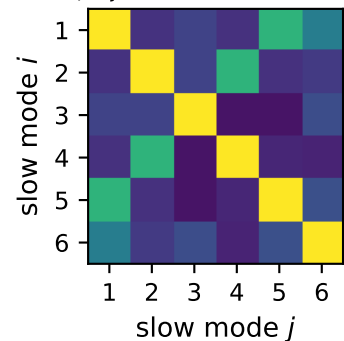
|v_i^H v_j| — top |\lambda| modes
