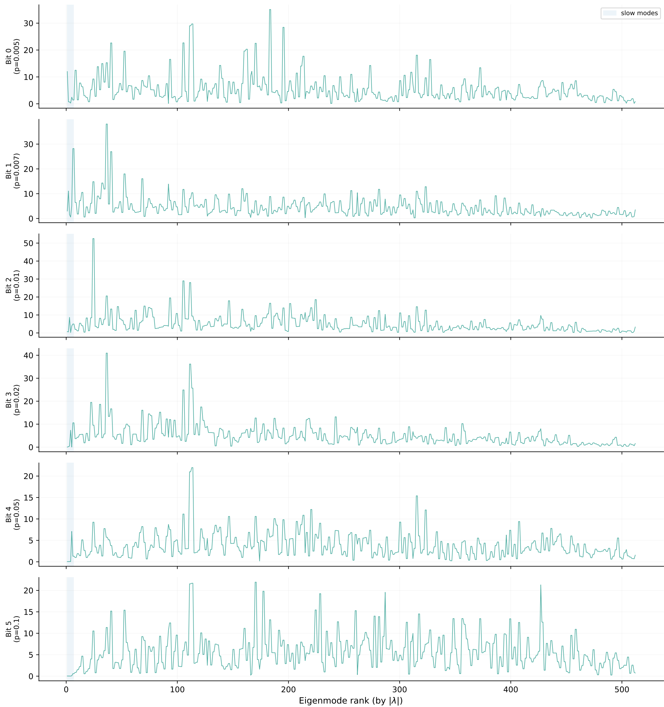
|V^{-1}W_{\text{in}}| — Input-to-mode coupling, g = 0.8
