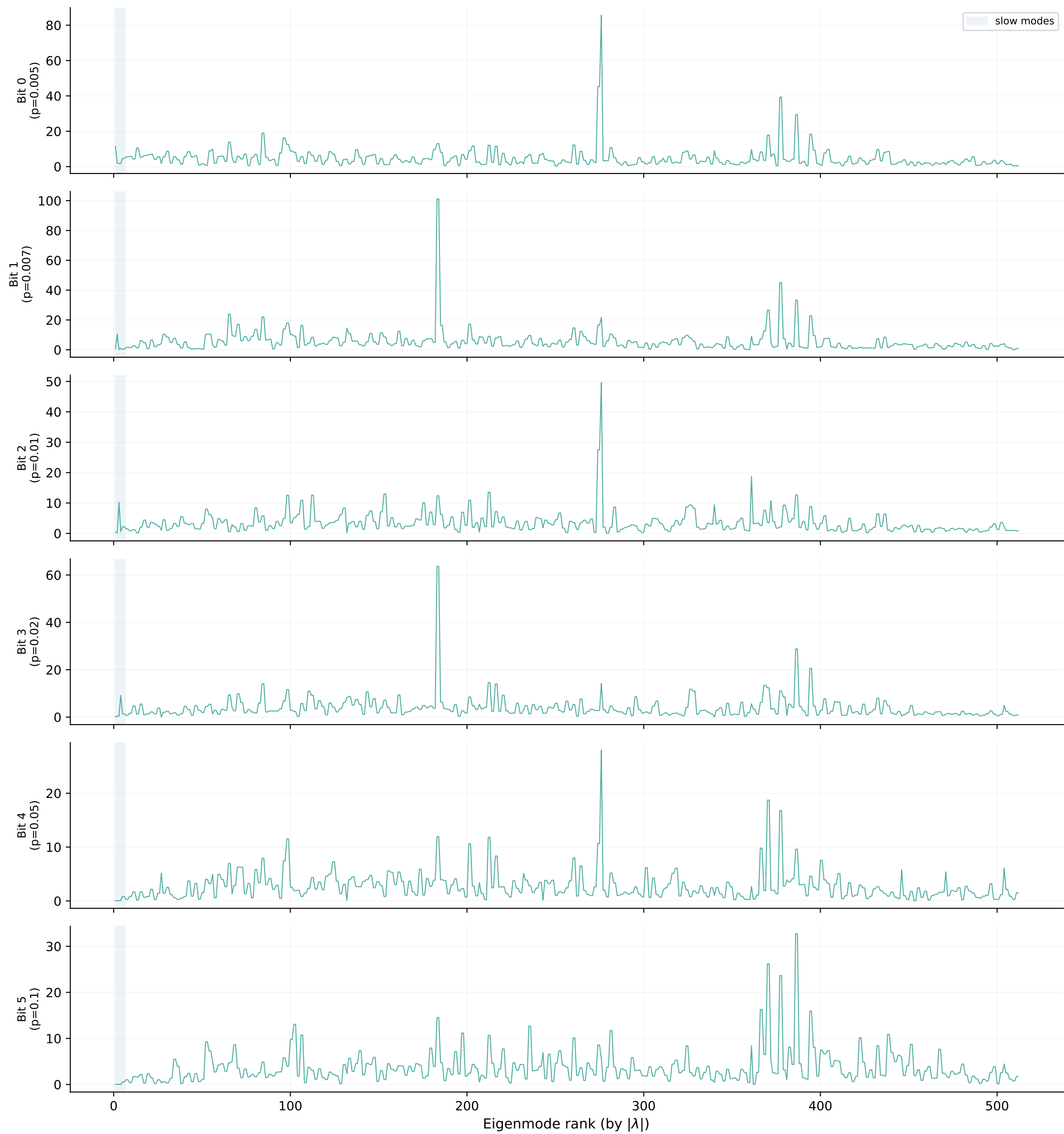
|V^{-1}W_{\text{in}}| — Input-to-mode coupling, g = 0.99
