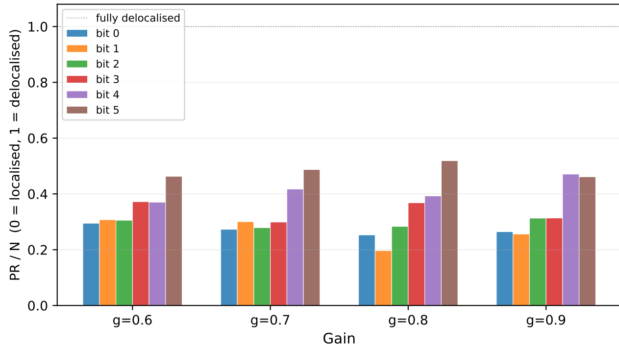
Fixed \tau = 1
