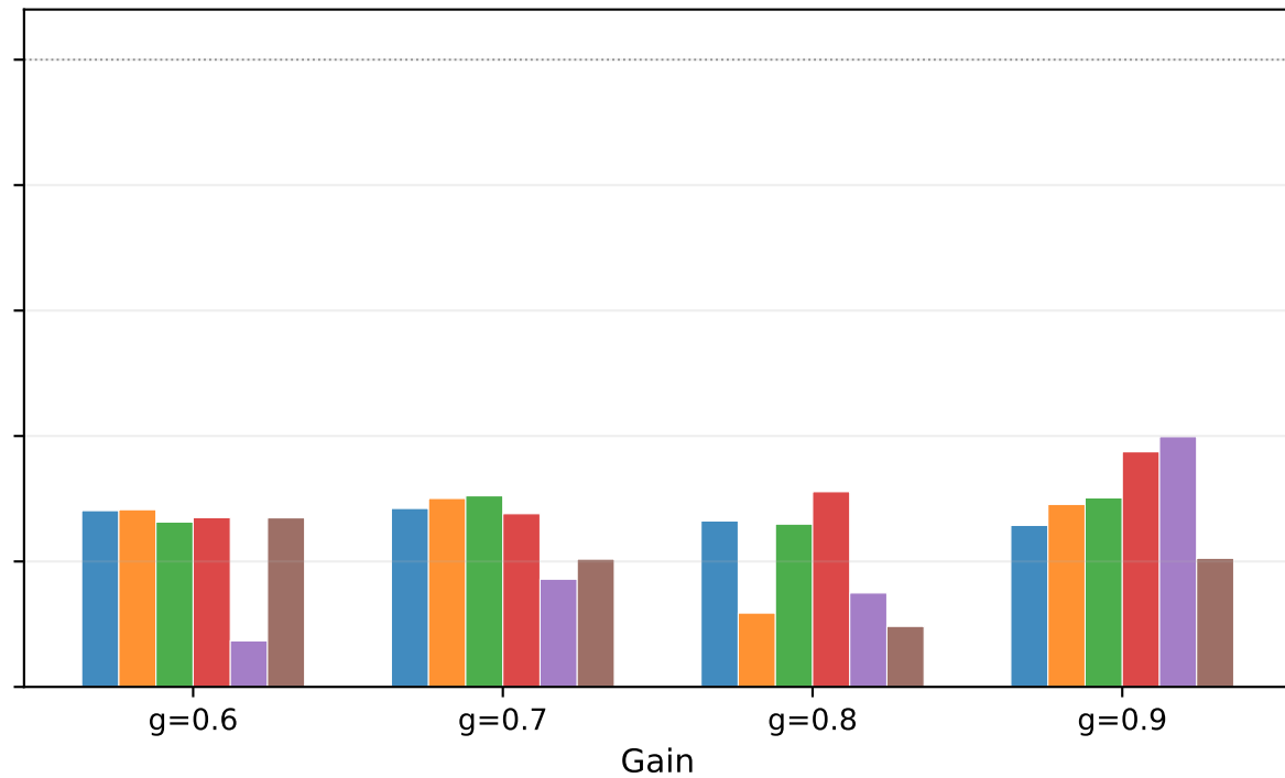
Learnable \tau
