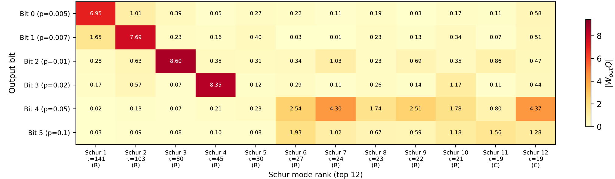
Learnable \tau ( g=0.6 \text{acc}=0.948 )
