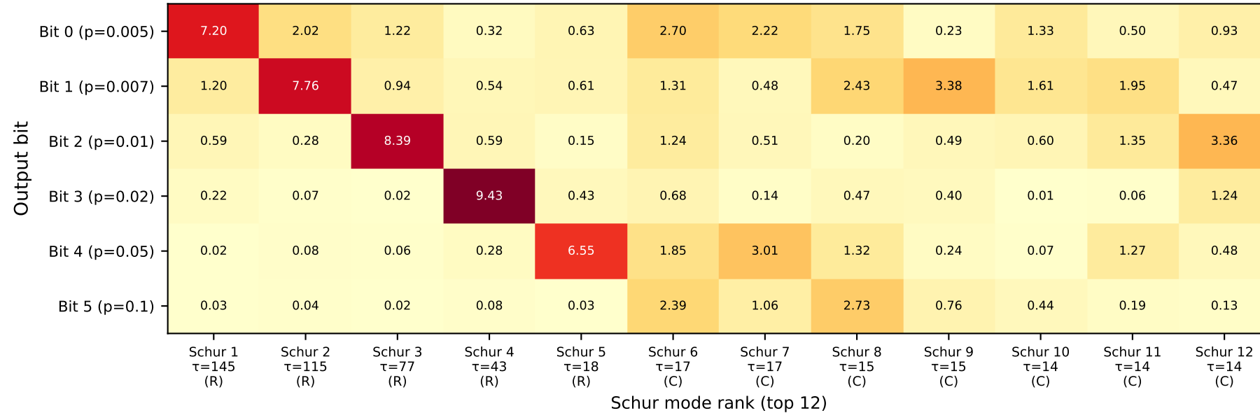
Fixed \tau = 1 ( g=0.6 \text{acc}=0.947 )
