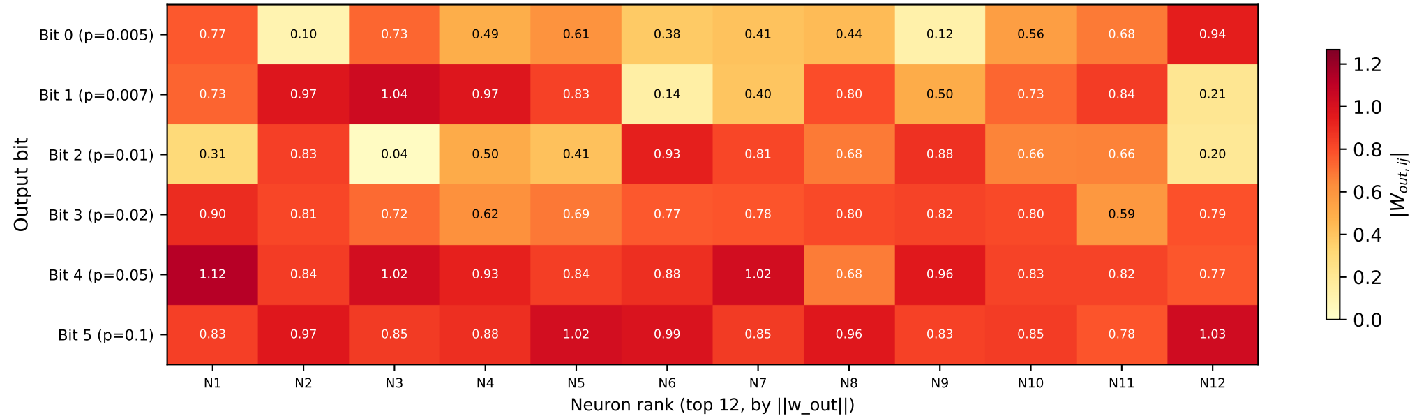
Fixed \tau = 1 ( g=0.6 acc=0.947 )
