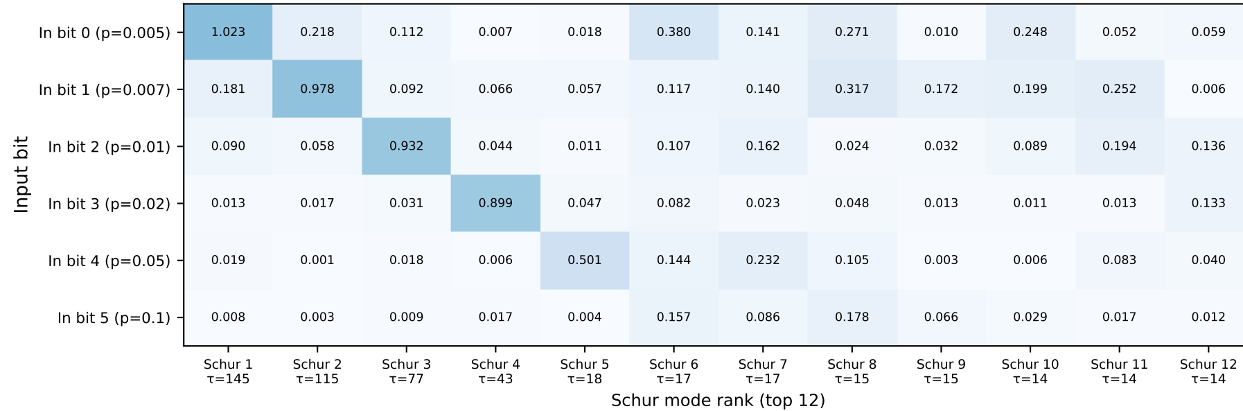
Fixed \tau = 1 (g=0.6 acc=0.947)
