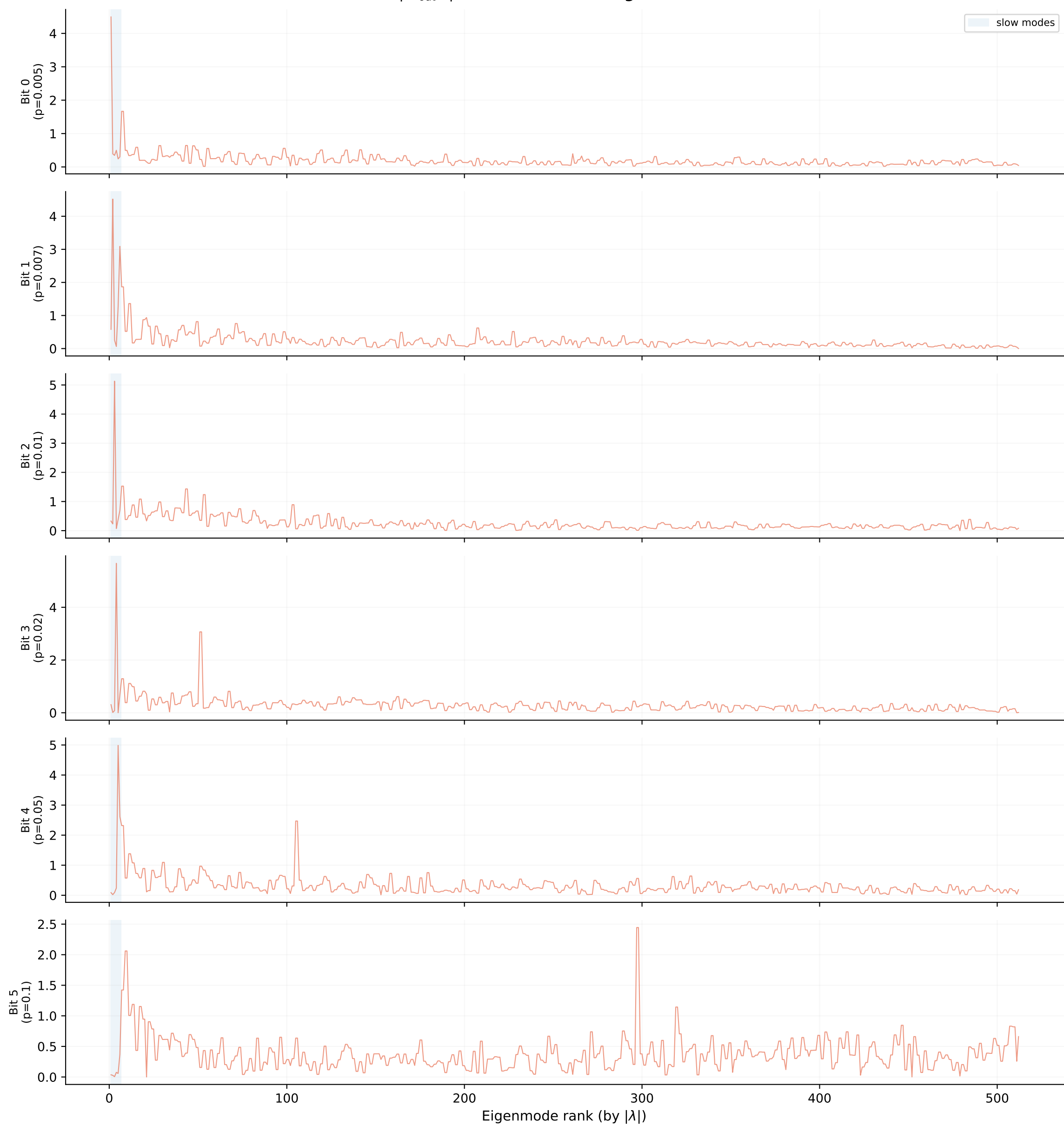
|W_{\text{out}} V| across all modes — g = 0.6
