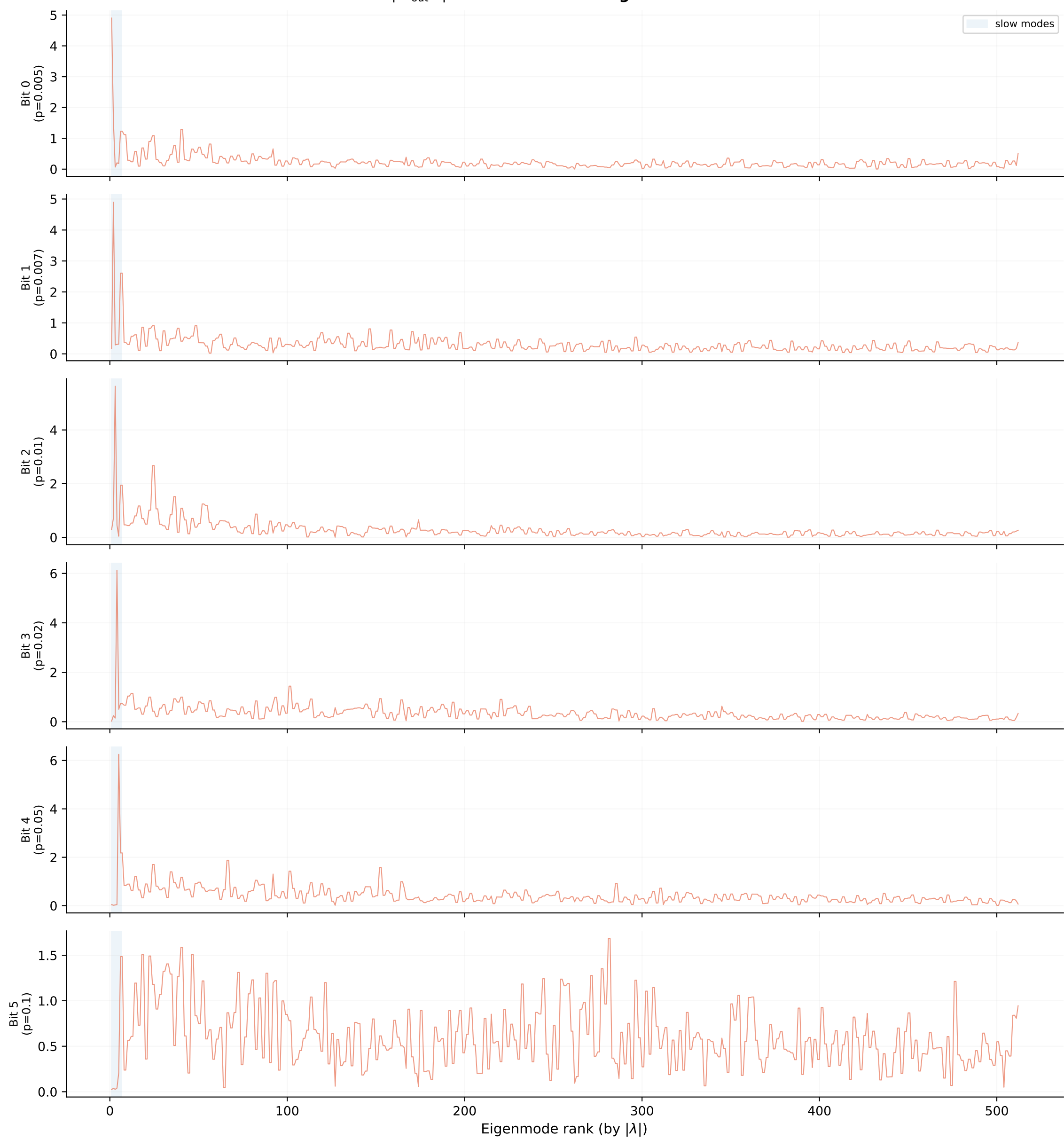
|W_{\text{out}} V| across all modes — g = 0.8
