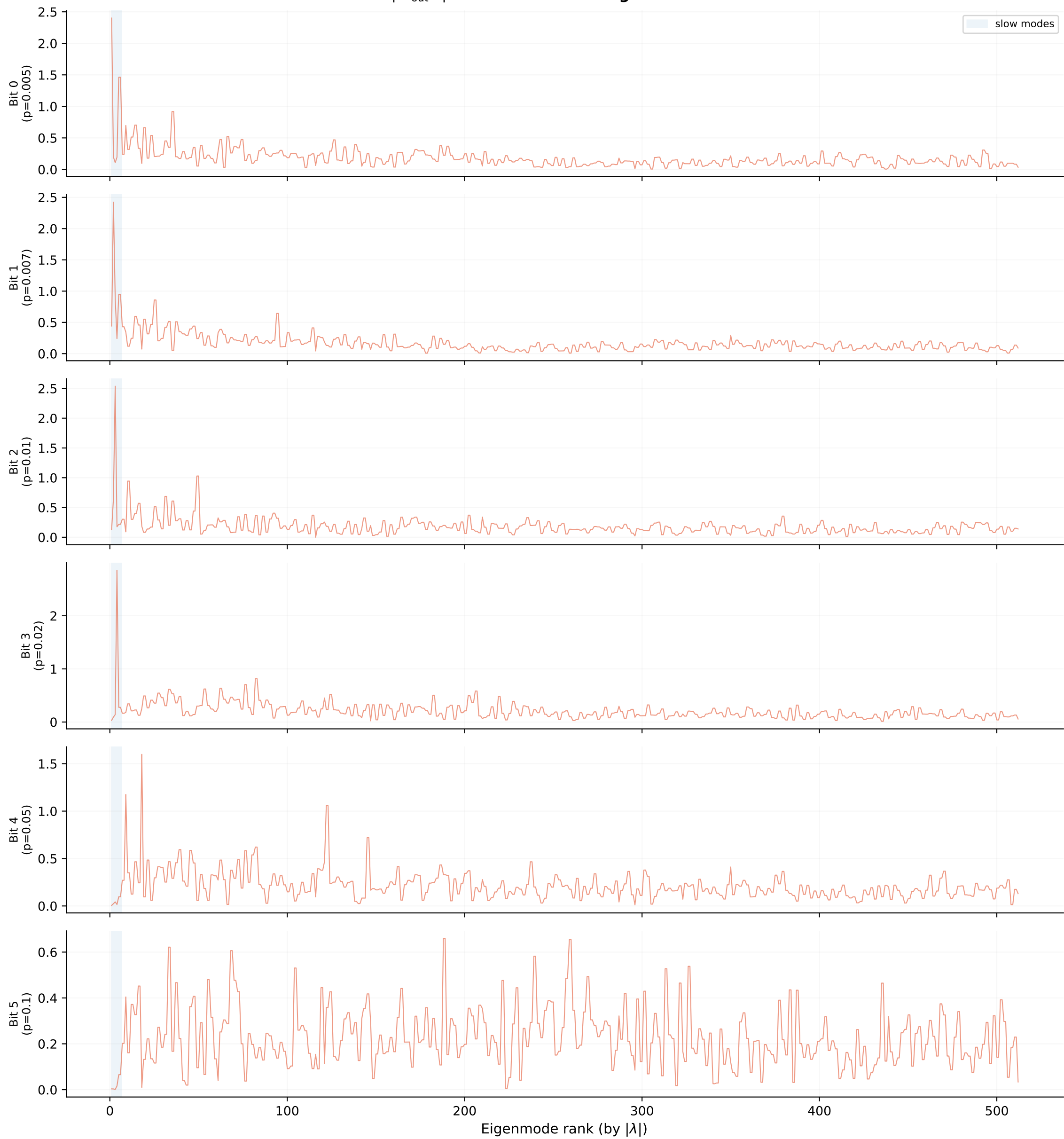
|W_{\text{out}} V| across all modes — g = 0.9
