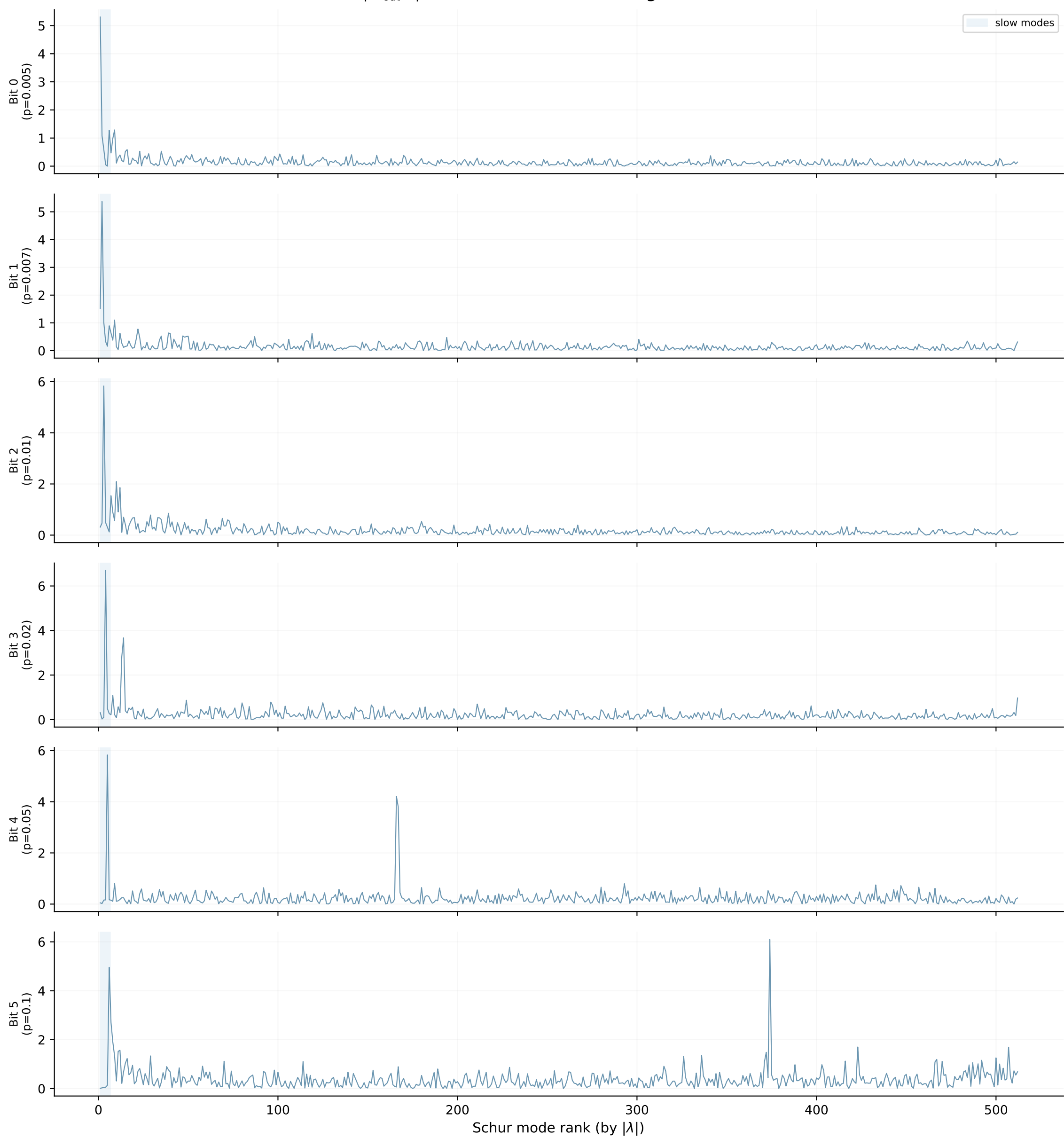
|W_{\text{out}} Q| across all Schur modes — g = 0.5
