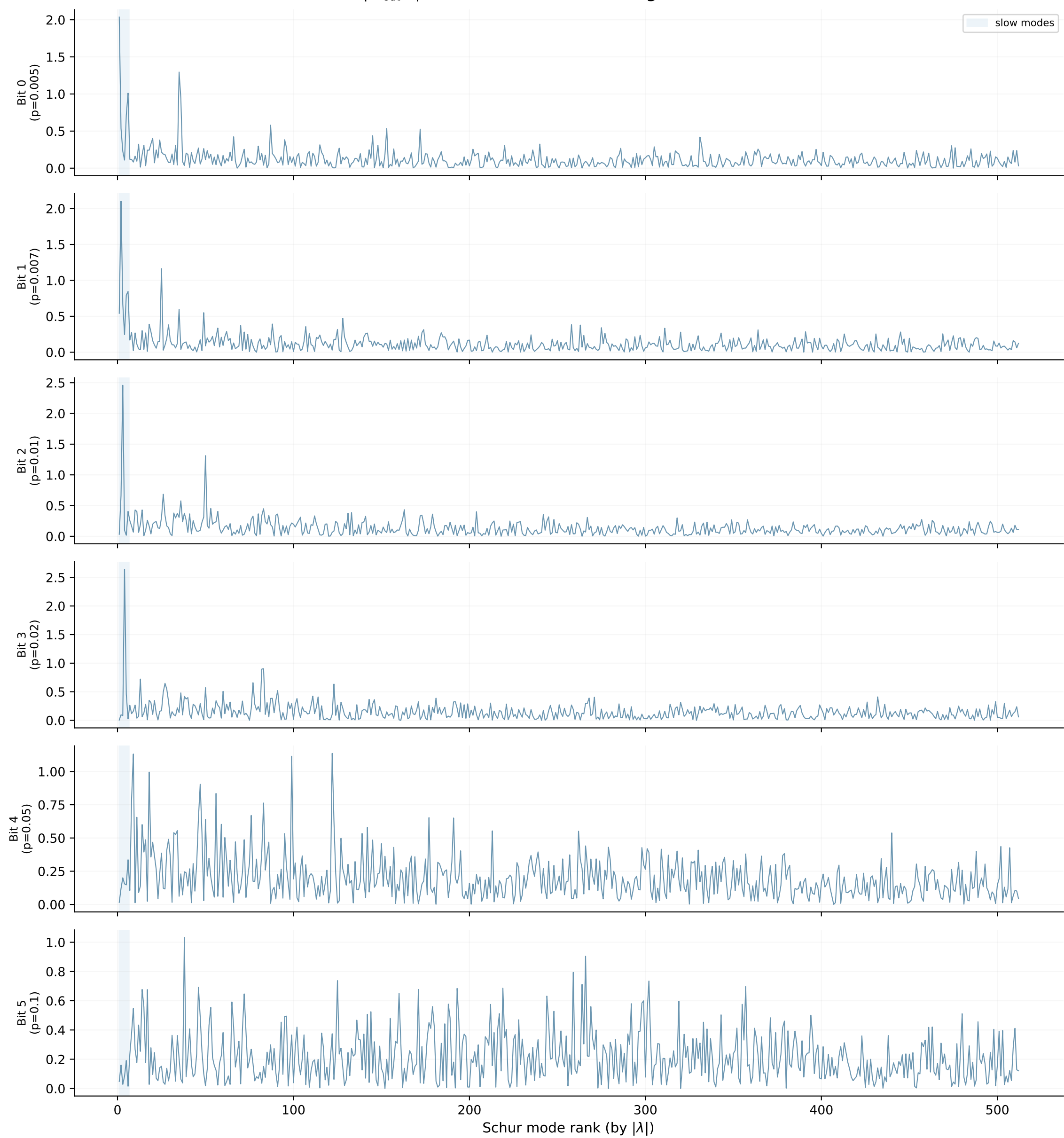
|W_{\text{out}} Q| across all Schur modes — g = 0.9
