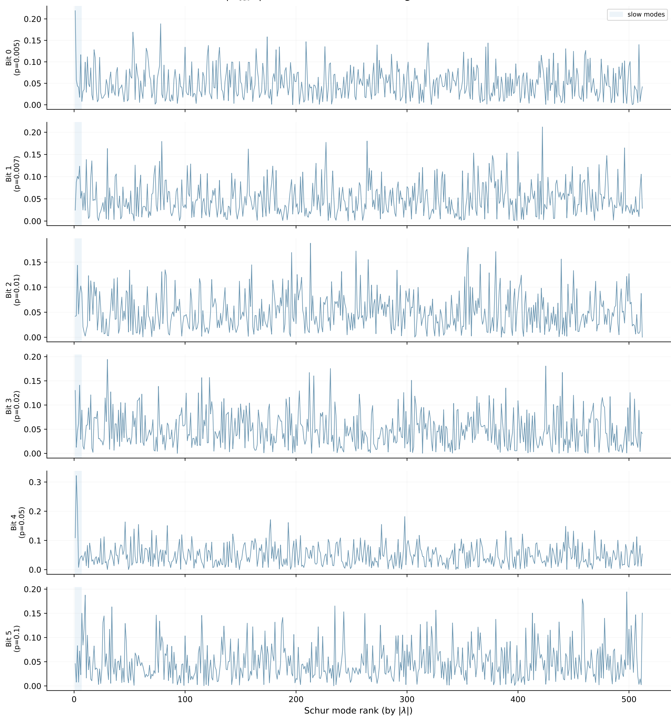
|W_{\text{out}} Q| across all Schur modes — g = 0.95
