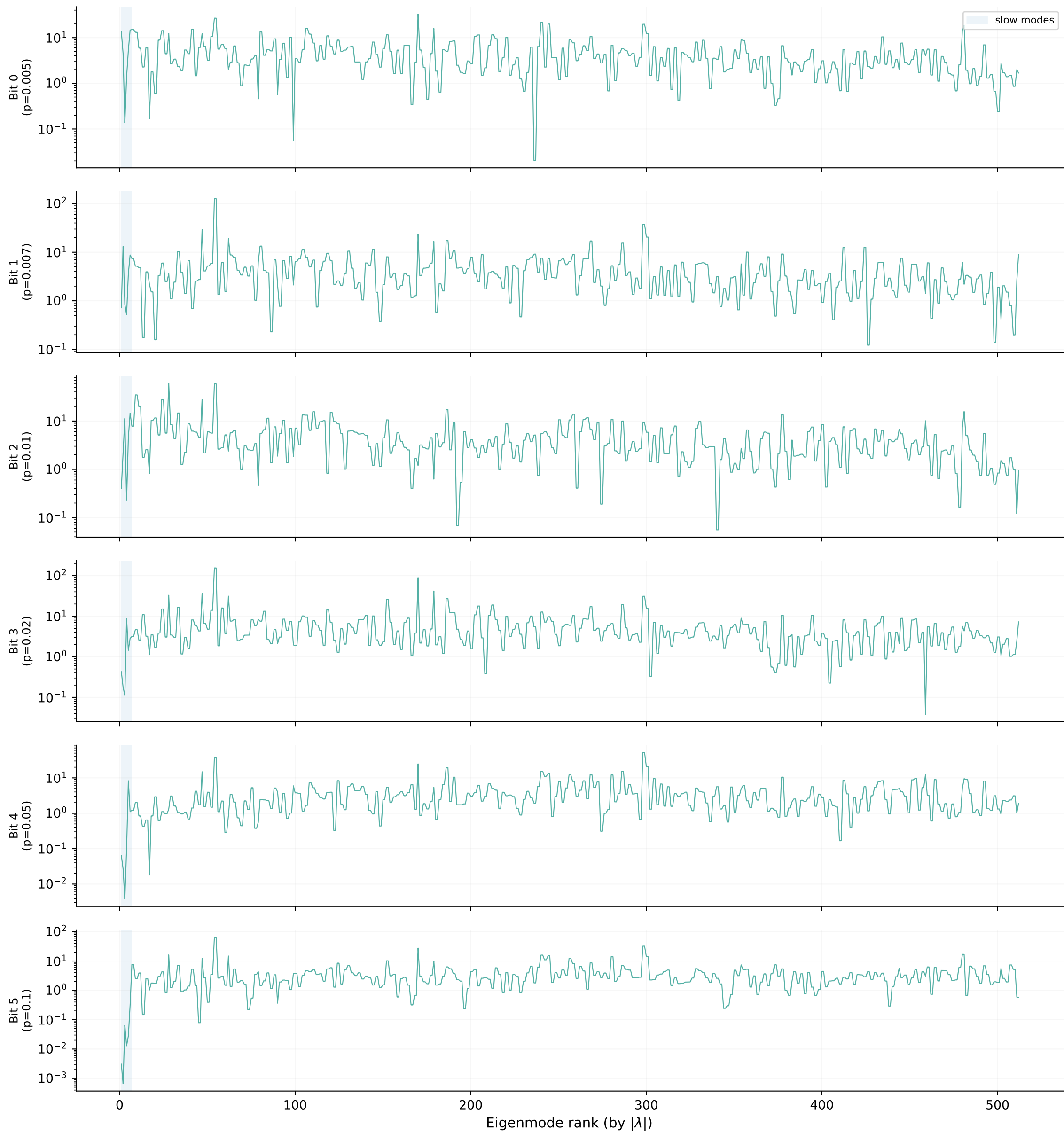
|V^{-1}W_{\text{in}}| — Input-to-mode coupling, g = 0.5
