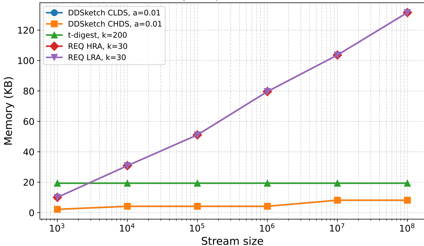
Memory Footprint, Pareto(1.5, 1)
