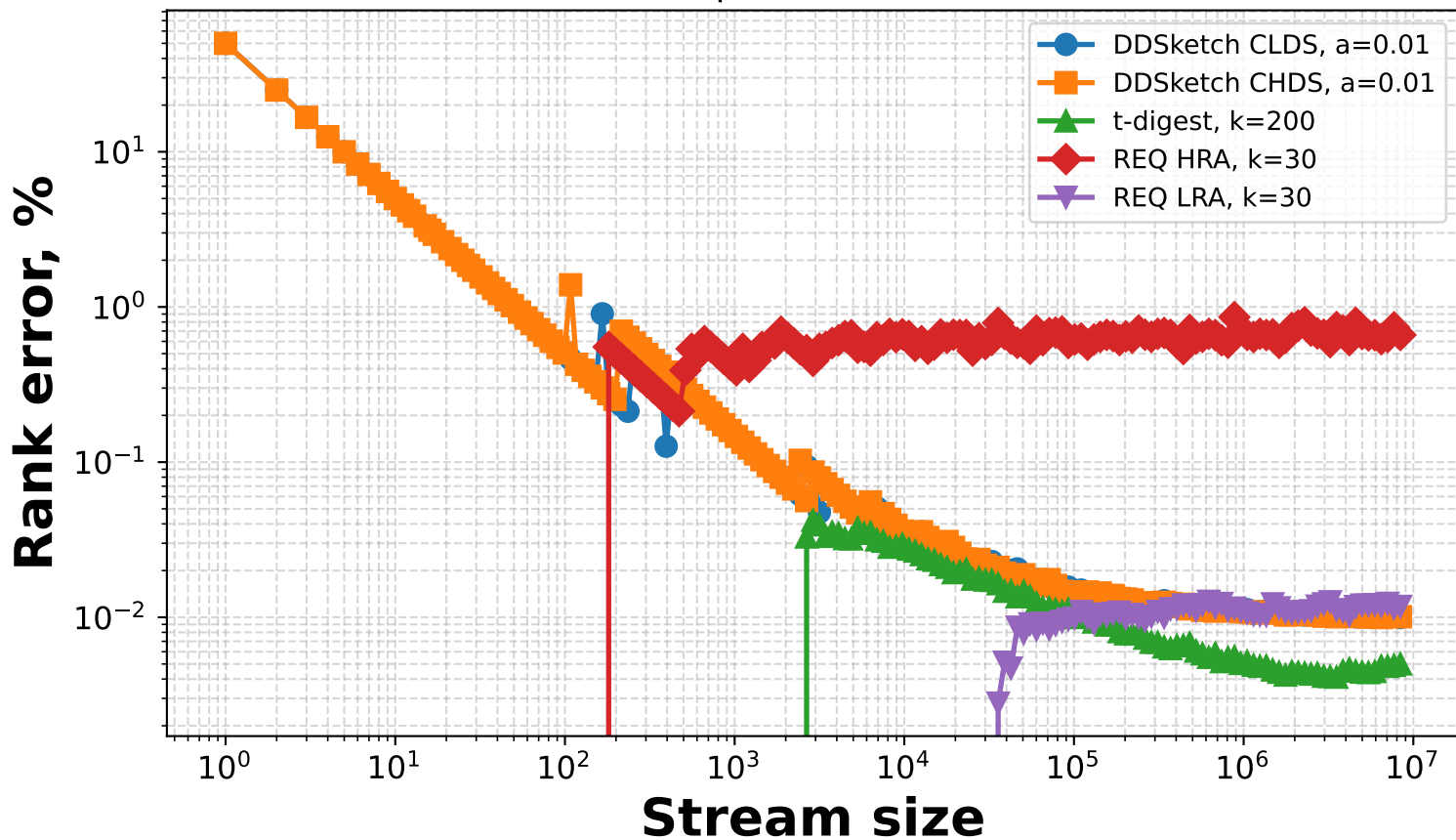
Rank Error, Exponential(1.5), rank 0.01
