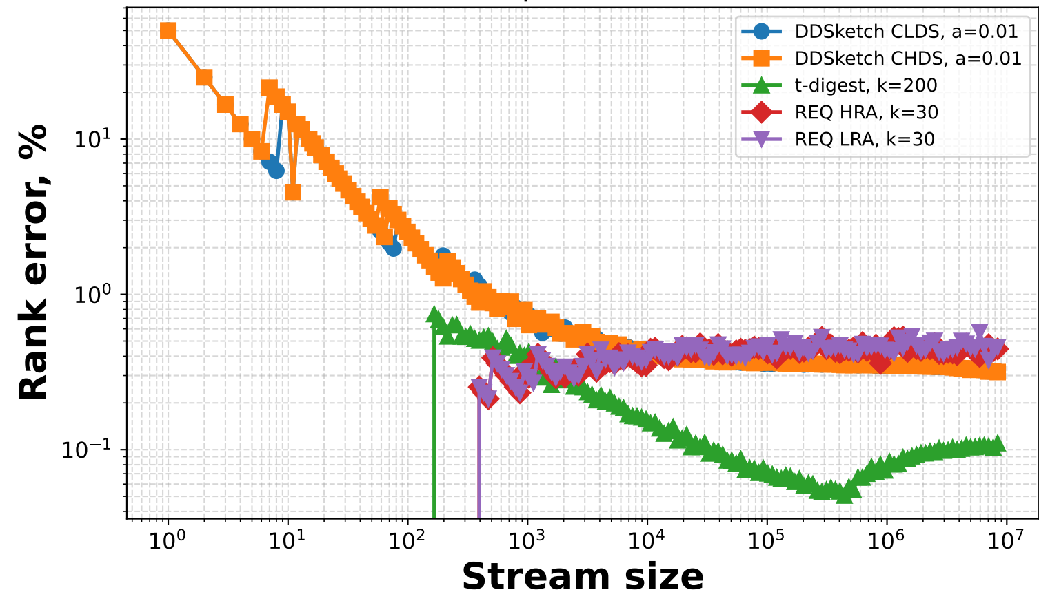
Rank Error, Exponential(1.5), rank 0.5
