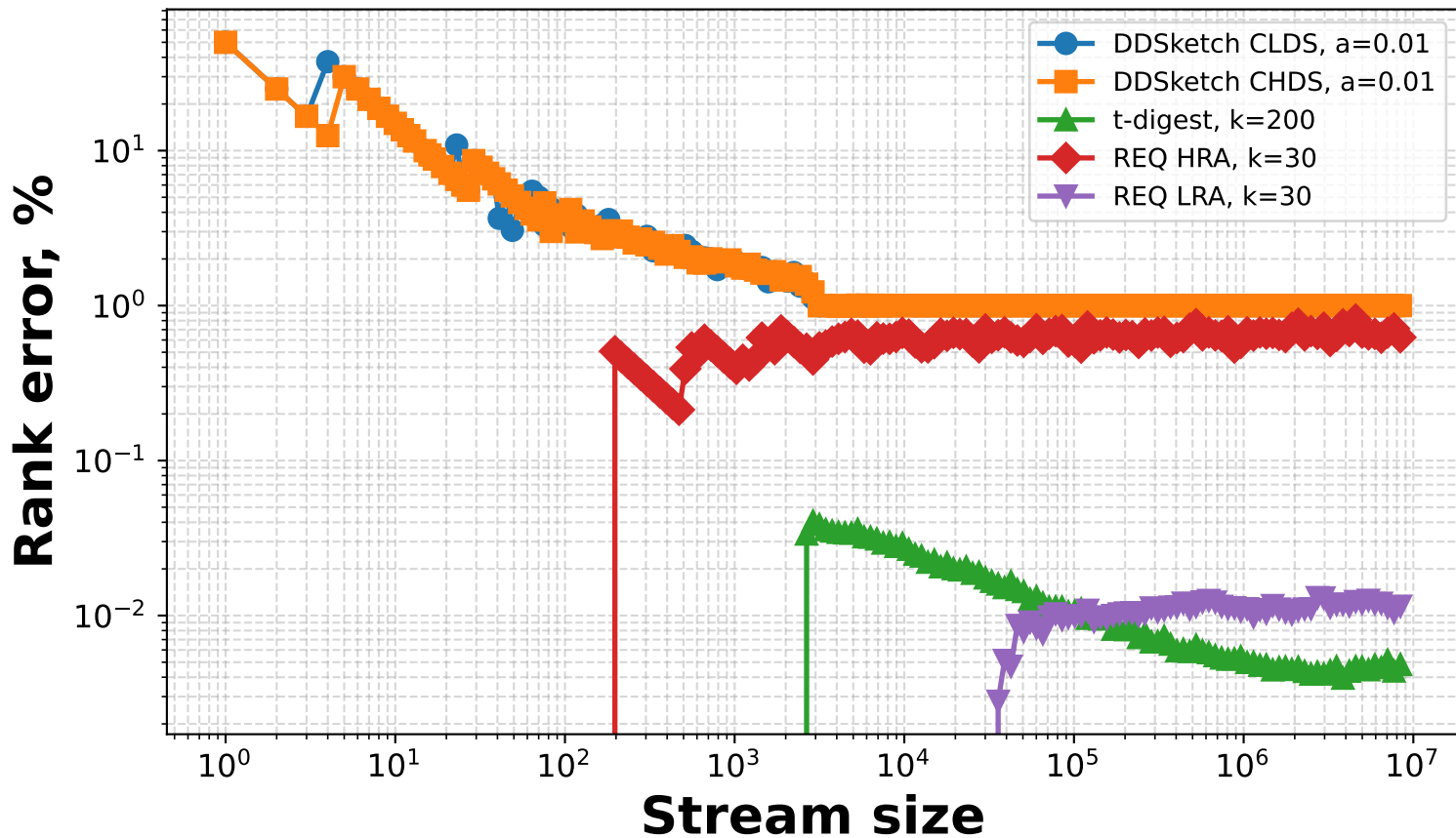
Rank Error, Pareto(1.5, 1), rank 0.01
