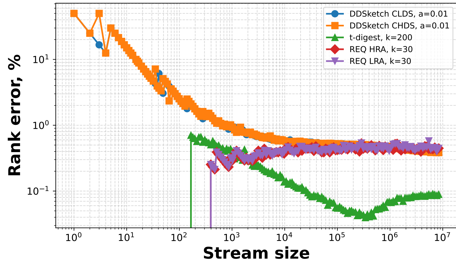
Rank Error, Uniform(0,1), rank 0.5
