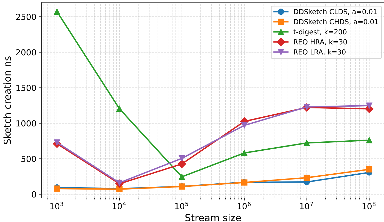
Sketch creation ns, Pareto(1.5, 1)
