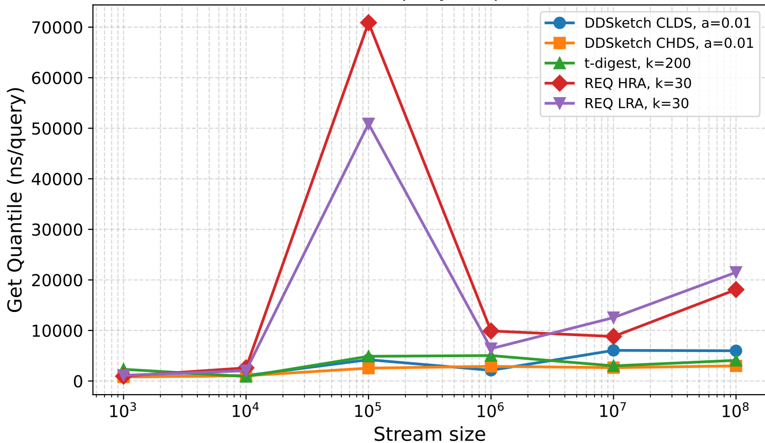
Get Quantile (ns/query), Exponential(1.5)
