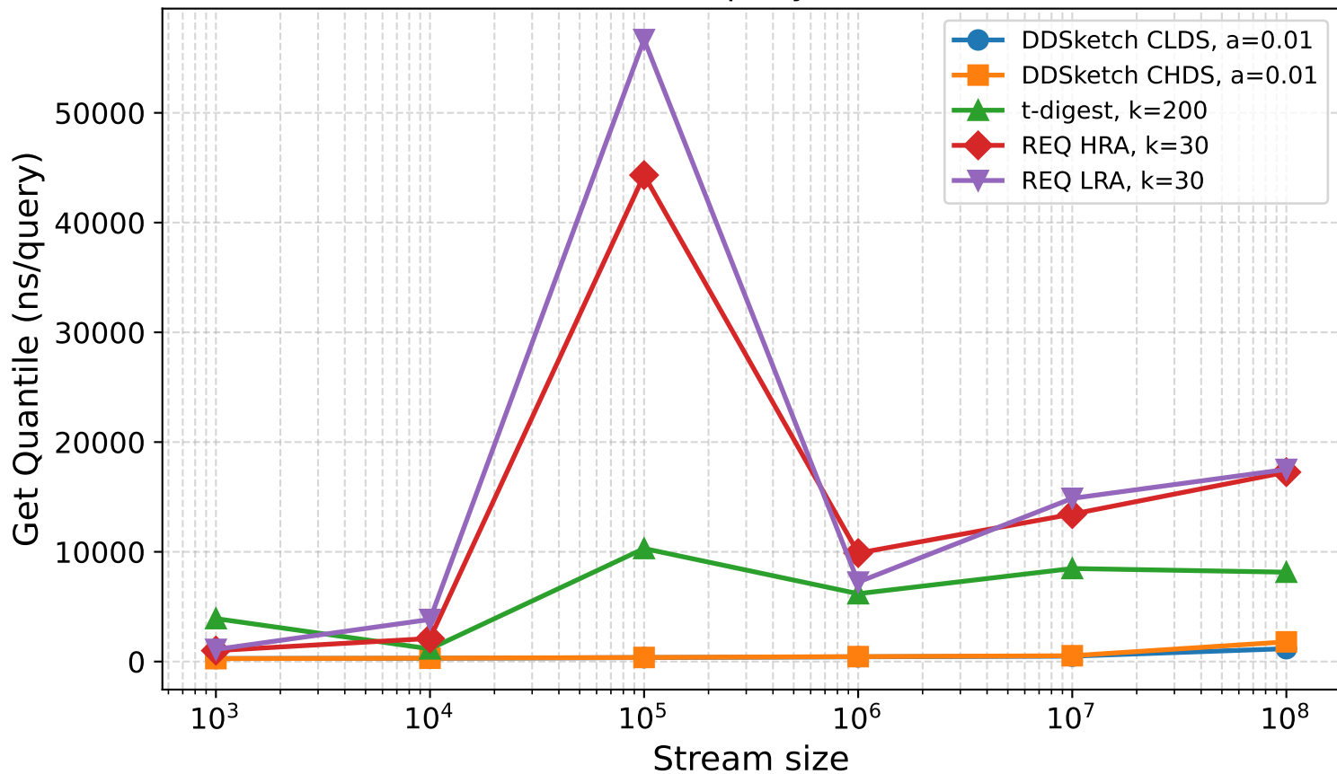
Get Quantile (ns/query), Pareto(1.5, 1)
