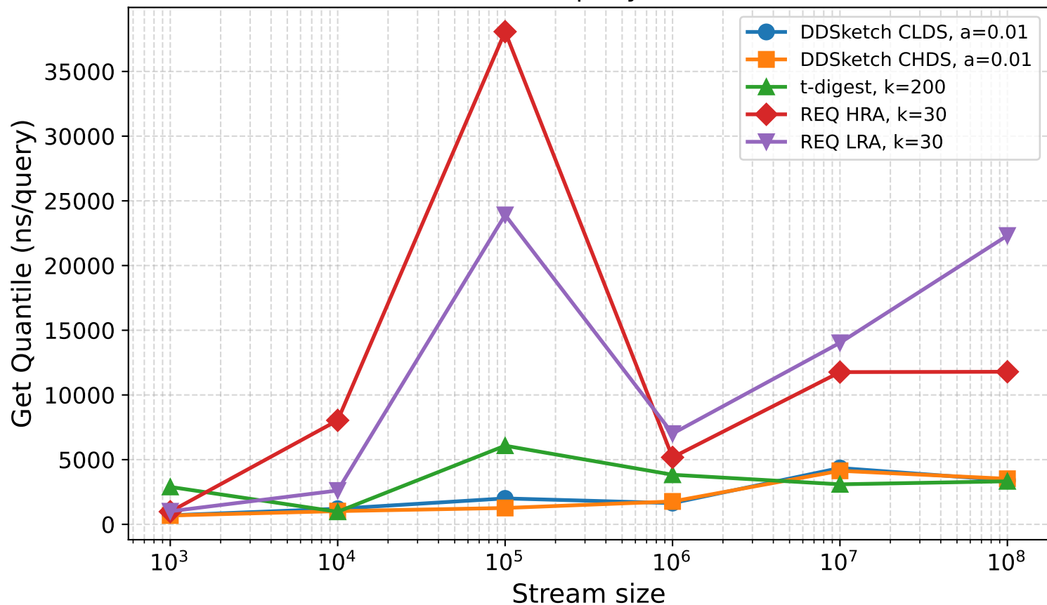
Get Quantile (ns/query), Uniform(0,1)
