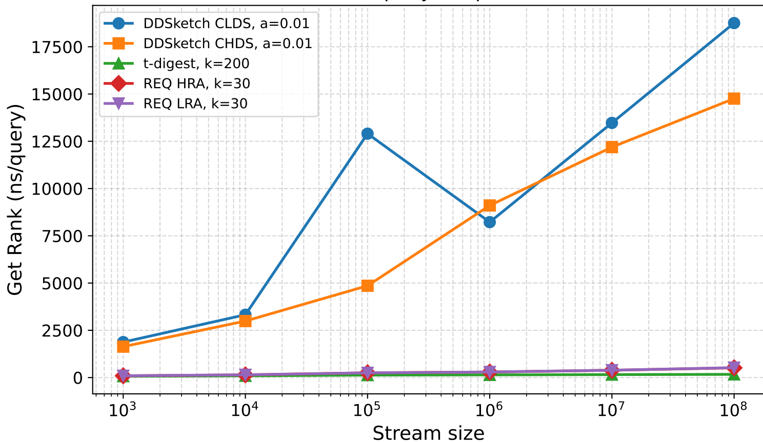
Get Rank (ns/query), Exponential(1.5)
