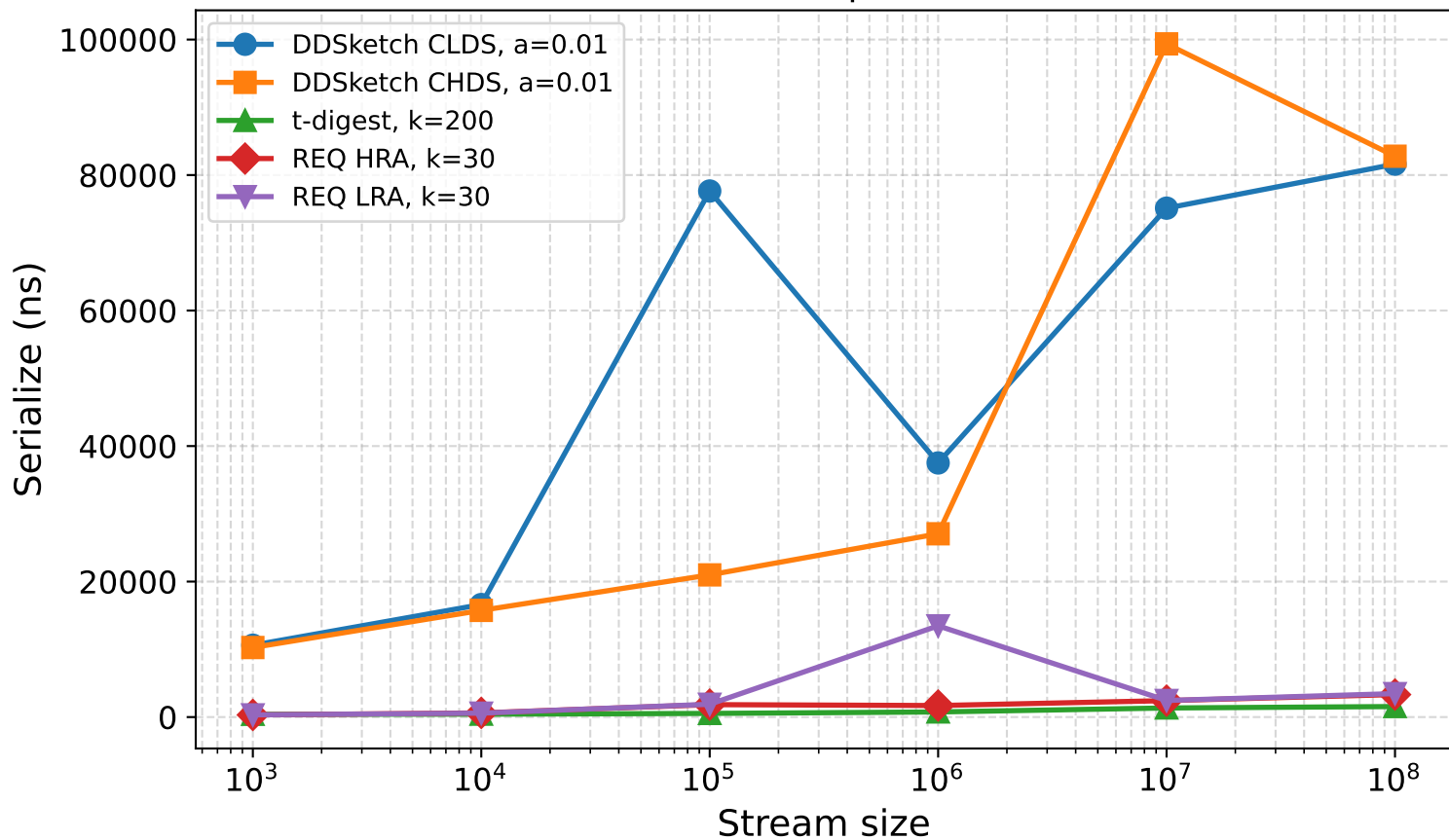
Serialize (ns), Exponential(1.5)
