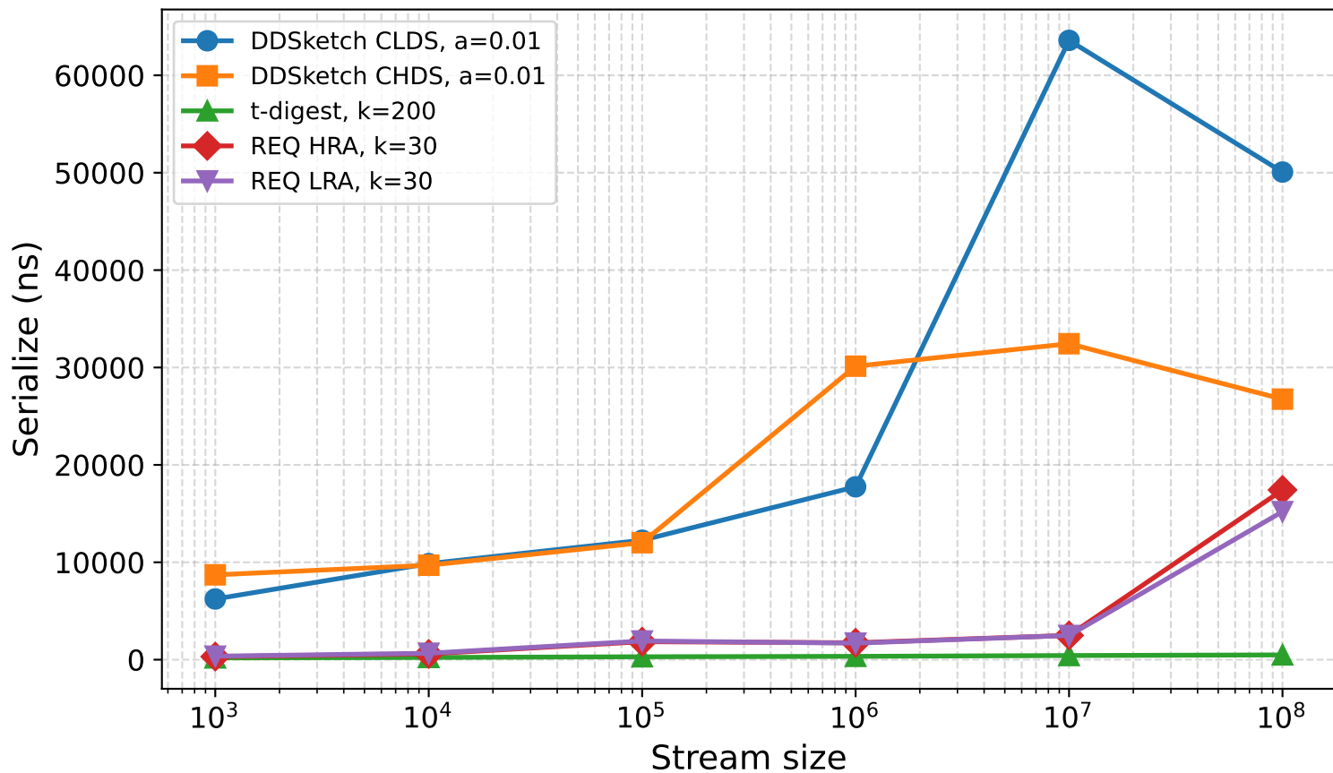
Serialize (ns), Pareto(1.5, 1)
