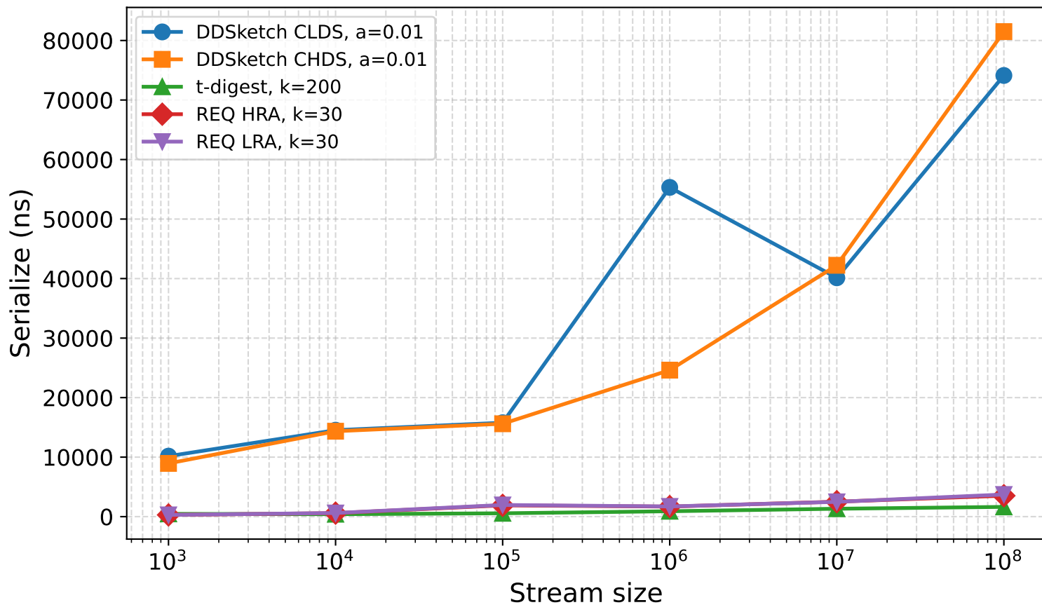
Serialize (ns), Uniform(0,1)
