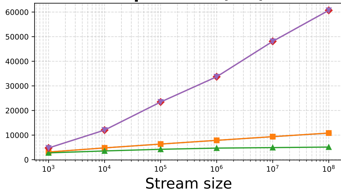
Exponential(1.5)
