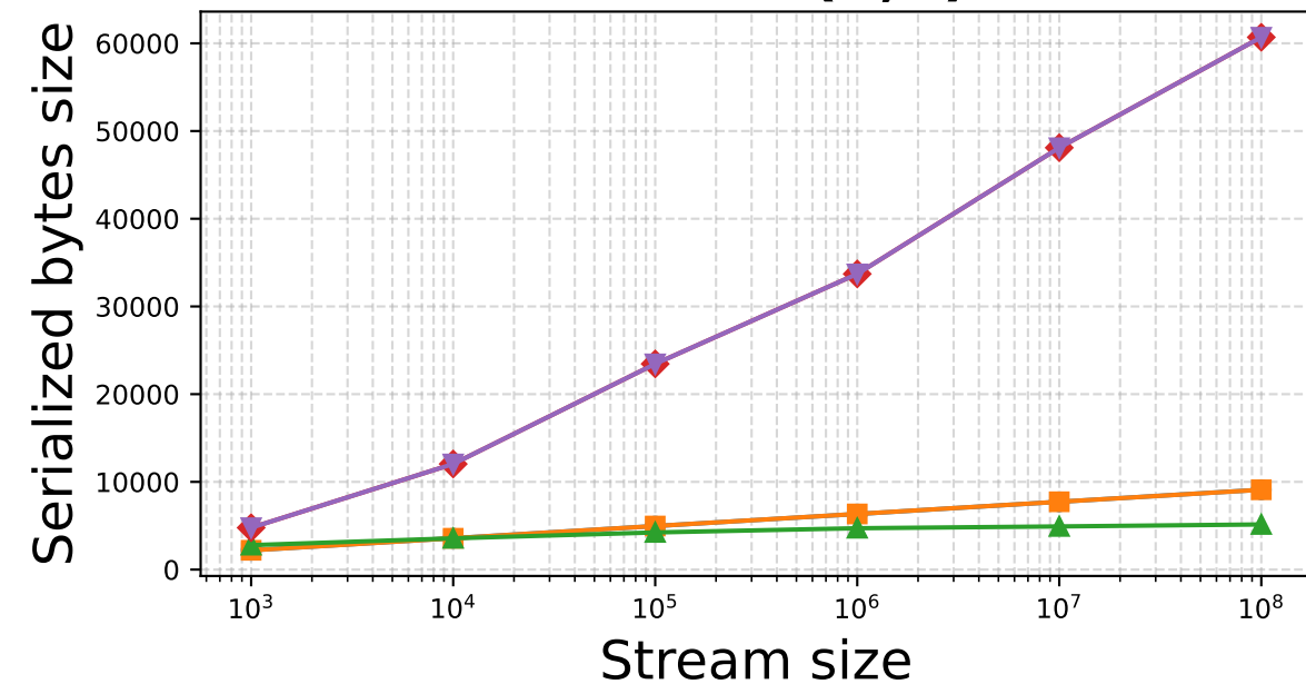
Uniform(0,1)
