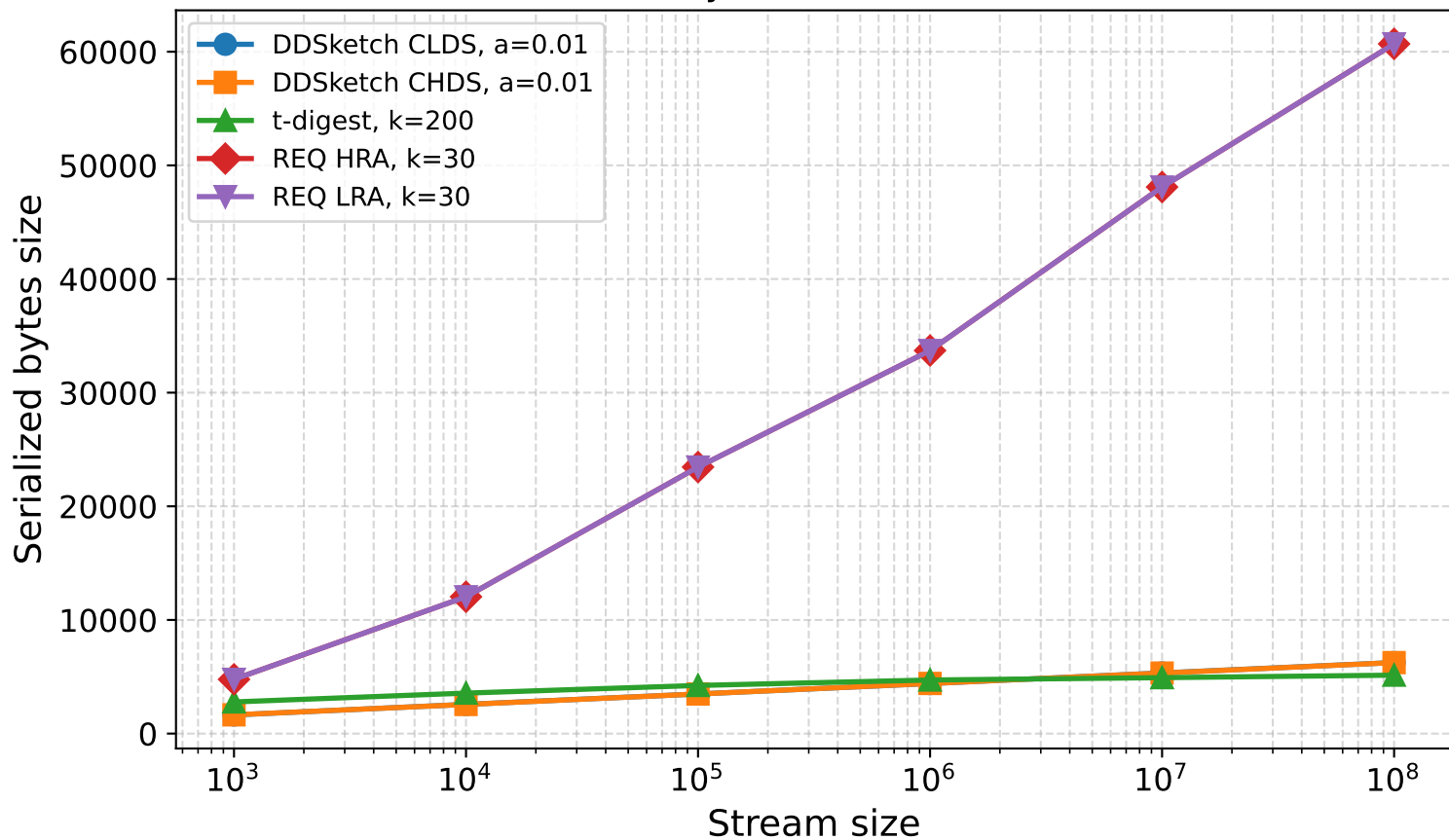
Serialized bytes size, Pareto(1.5, 1)
