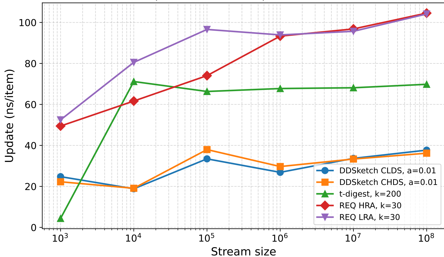
Update (ns/item), Exponential(1.5)
